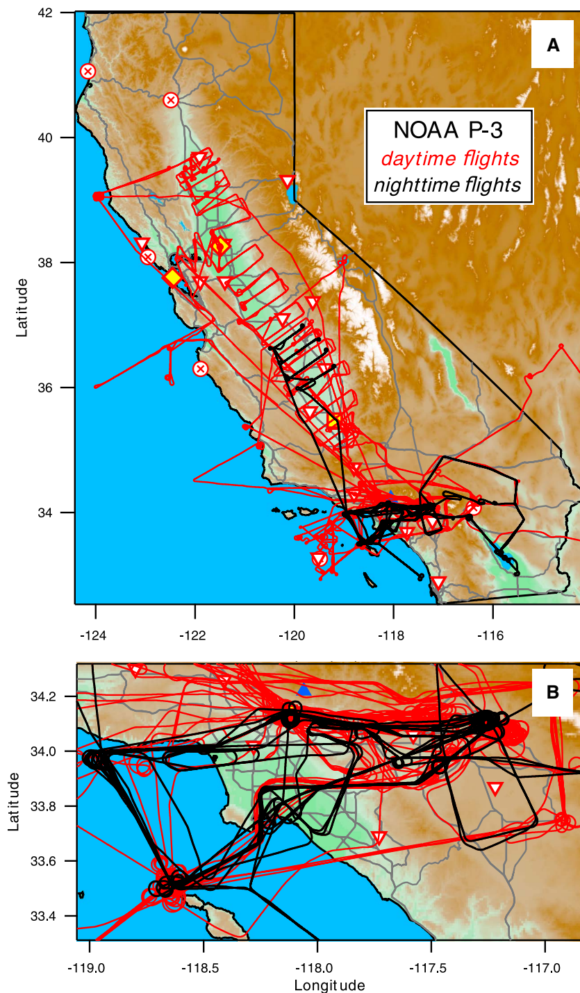
Figure 3. (a) Daytime (red lines) and nighttime (black lines) NOAA P-3 research aircraft flight tracks in California between 30 April and 22 June 2010. (b). As in Figure 3a, showing details of P-3 flight segments within the South Coast Air Basin.
